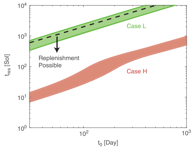
FIG. 6. Parameter ranges for the local atmospheric residence time of methane ( t_{\text{res}} ) and the baseline residence time of soil carbon ( t_0 ) that produce a 7 \pm 2 ppb methane spike at \text{LS} \sim 100^\circ as measured by MSL. (Color graphics available at www.liebertonline.com/ast )
