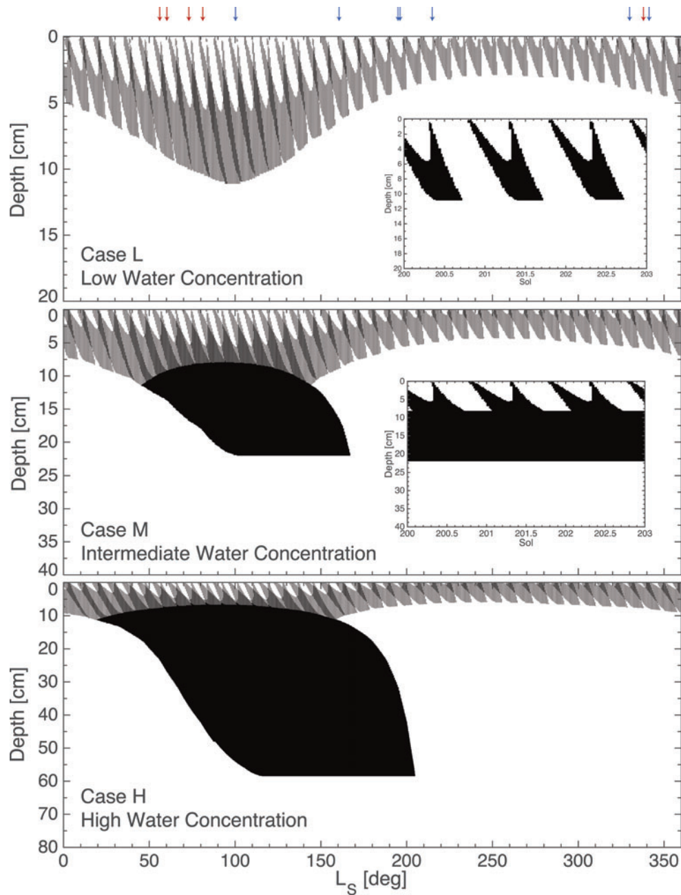
FIG. 3. Subsurface layers in which deliquescent perchlorate solution is expected. The depth range in which calcium perchlorate salts are deliquescent and forming liquid brine is shown in black. The three panels correspond to three cases for daytime water concentration. Note different vertical scales among the panels. The two inserts provide zoom-in views of 3 sols to illustrate the diurnal cycle of deliquescence and efflorescence in the shallow subsurface. The arrows on the top indicate the L_S when SAM's methane measurements were taken, with the blue arrows indicating background measurements and the red arrows indicating the spike measurements. (Color graphics available at www.liebertonline.com/ast )
