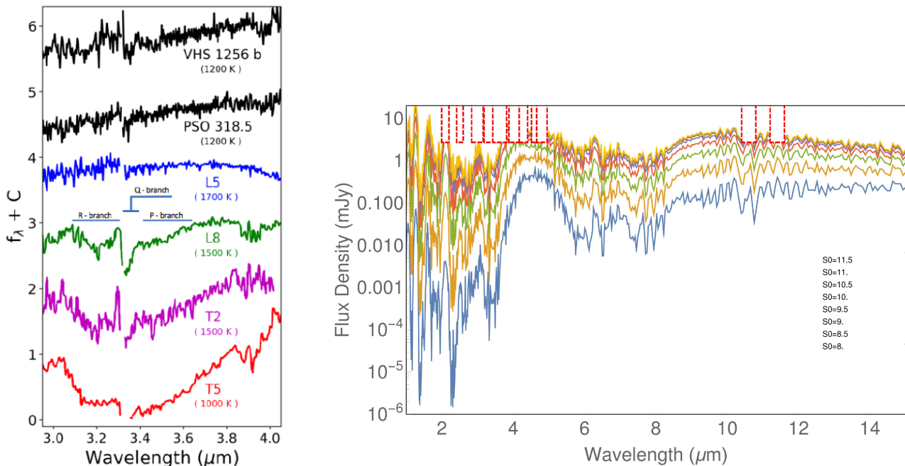
Fig. 2.— left) JWST spectra will reveal the presence of molecules such as \text{H}_2\text{O} , \text{CO} , \text{CH}_4 , \text{NH}_3 . Ground based spectra of two low gravity analogs to the HR8799 planets (VHS1256b (ID#1386) and PSO 318.5) and a range of L and T dwarfs suggest the power of spectroscopy (here using \text{CH}_4 ) to characterize atmospheric properties such as vertical mixing and non-equilibrium chemistry. right) Illustrative model spectra of a 2 Myr old, 2 M_{Jup} planet at 10 pc for a number of different initial entropy values (“hot start” to “cold start” (Spiegel and Burrows 2012). Red rectangles at the top show a number of NIRCcam and MIRI filters. MIRI will study young planets at wavelengths longward of 5 \mu\text{m} for the first time.
